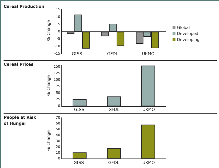
Figure 1. Estimated effects of climate change in 2060 on cereal production, cereal prices and risk of hunger. Reference case without climate change assumes: Cereal production = global 3 286 mmt, developed 1 449 mmt, developing 1 836 mmt. Cereal prices 1970 = 100. People at risk of hunger = 641 million.
