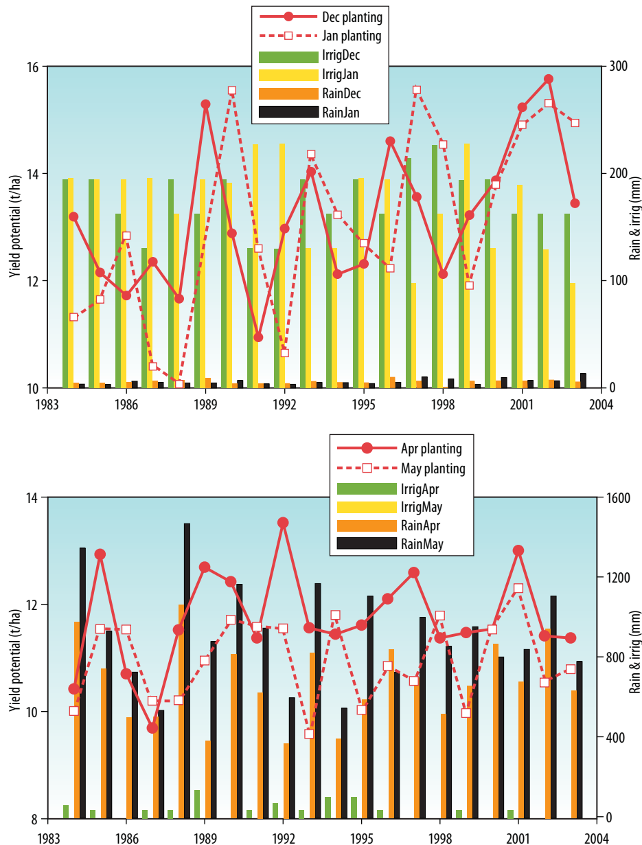
Figure 15. Variability of simulated yield potential and irrigation water requirements for growing Kharif-1 season (April - May planting) or Rabi season (Dec. - Jan. planting) maize (hybrid maturity: 1600 GDD) at Bogra, Central North Bangladesh.
