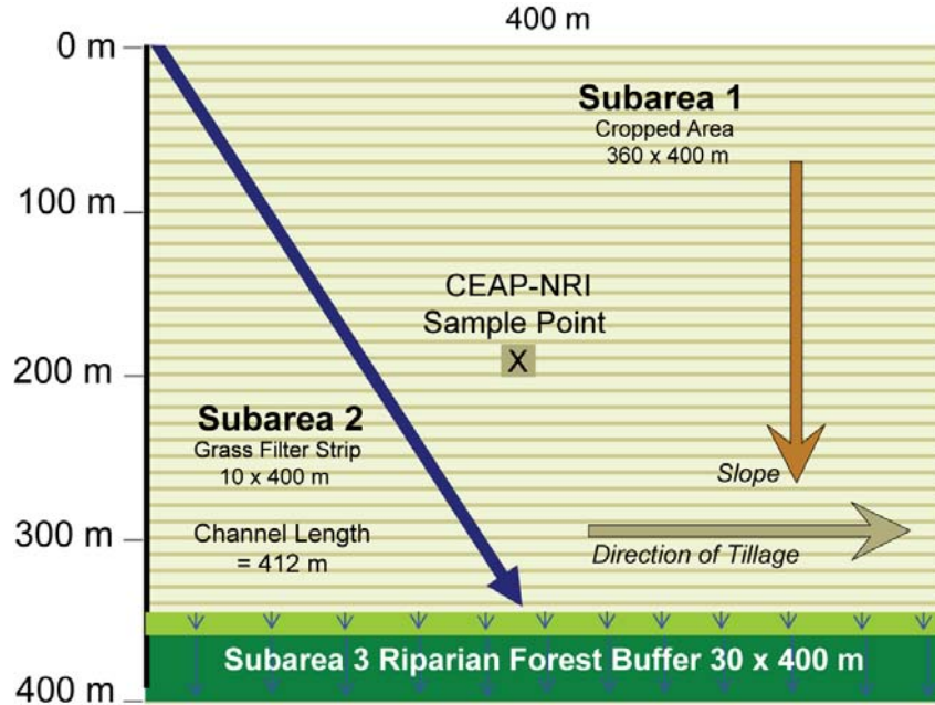
Figure 42. APEX field configuration used to represent a riparian buffer for CEAP National Assessment, shown with tillage performed on the contour (Source: BREC, 2008)
