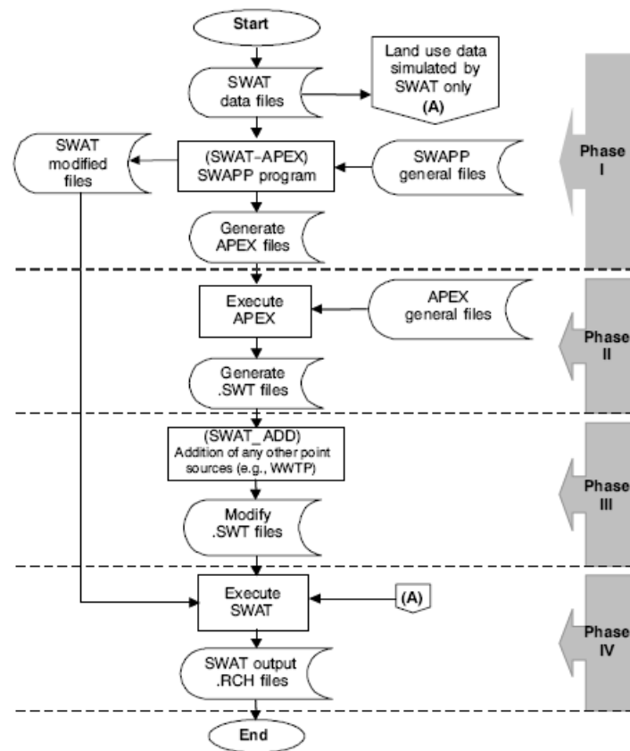
Figure 45. Schematic showing the four main phases of a SWAT-APEX (SWAPP) program application (Source: Saleh and Gallego, 2007)
