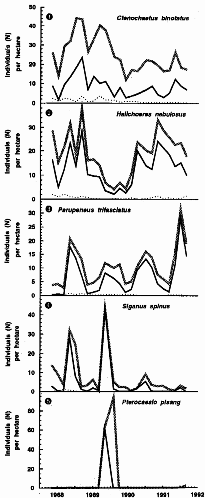
Fig. 3.8. Abundances of the most common species in the reef slope visual censusing (grey = combined sizes, black = recruits, dotted = adults). Fish drawings are by Magnus Olsson-Ringby.
