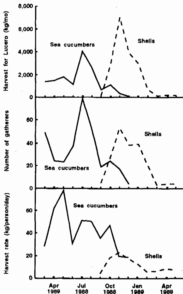
Fig. 2.11. Harvest data on sea cucumbers and shells from Lucero on Santiago Island. The alternation of seasons leads to shifting occupations among some harvesters. Data are from a survey by de Guzman (1990).
