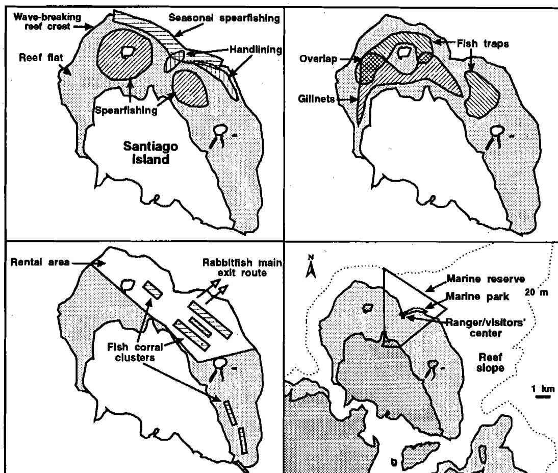
Fig. 6.2. Marine reserve/park system relative to primary reef flat fishing areas. The eastern corner of the reserve would bisect the major migration path for Siganus fuscescens (barangen), ensuring a supply of adult fish for the gillnetters and spearfishers, and still permitting substantial harvests for the fish corral owners.
