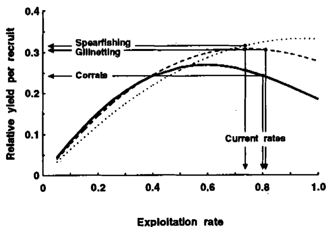
Fig. 6.3. Yield-per-recruit analysis for Siganus fuscescens (barangen). Curves show that the fine-meshed fish corrals induce growth overfishing far more than gillnets and spearfishing as locally utilized. Yields could be improved by favoring spearfishing over fish corrals. This would also improve income distribution because of the labor-intensive nature of spearfishing. Population parameters were based on monthly length histograms per gear weighted by annual catch and combined. Procedures followed those in del Norte and Pauly (1990), but involved an improved data set from mid-1988 to mid-1989 ( L_{\infty} = 26.0 , K = 0.84 , M = 1.71 ). Natural mortality was estimated from the Pauly environmental formula, using T = 30^{\circ}\text{C} . Individual catch curves by gear were used to estimate the length of first capture ( L_c ) per gear (Gayanilo et al. 1988).
