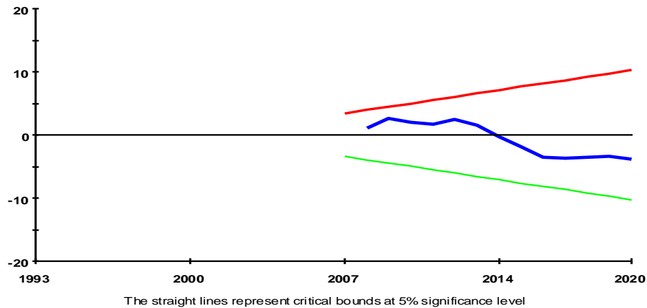
Figure 5: Plot of cumulative sum of recursive residuals
