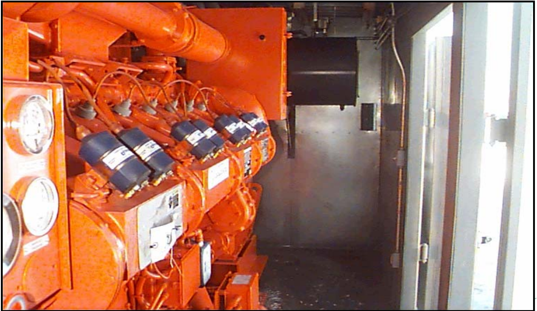
775 kW Waukesha engine
