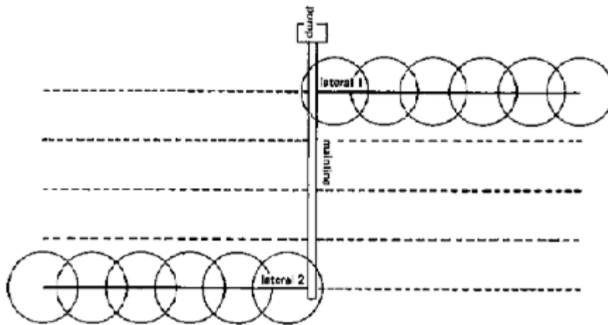
Figure 7.4: Example of layout for gun-spray sprinkler (Source: FAO, 1985)
