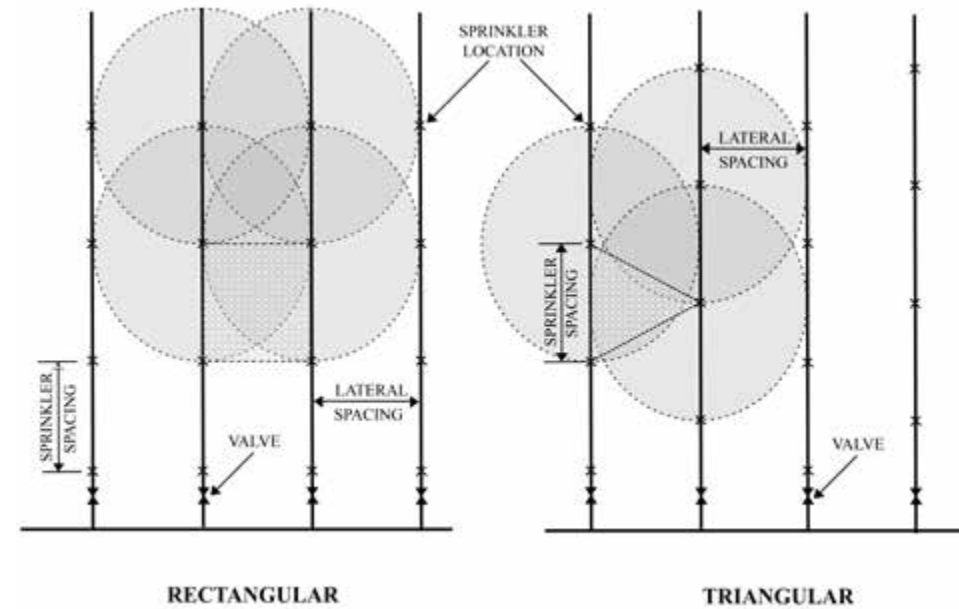
Figure 7.3: Sprinkler layout in rectangular or triangular arrangement (Source: Stephanie and Andrew, 2014)
