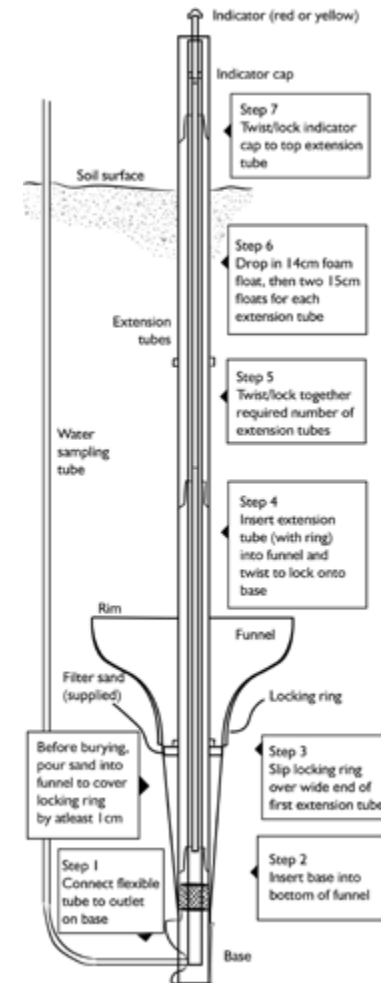
Figure 9.3. Installation steps
