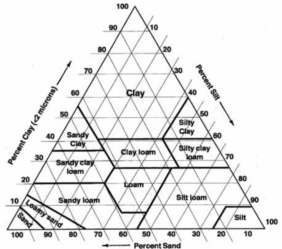
Figure 1.2: Soil textural classes
