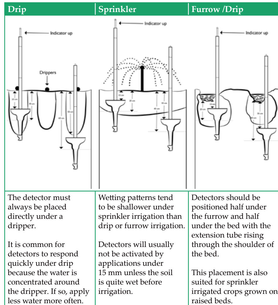
Figure 9. 4: Depth of placement of WFDs
