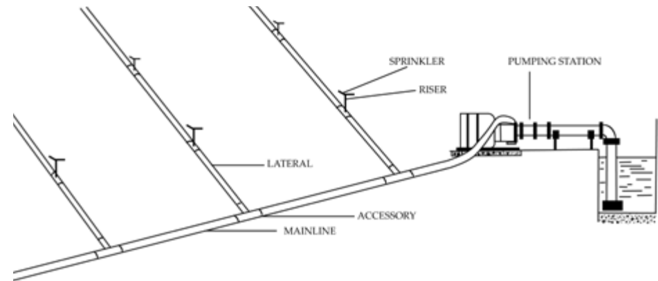
Figure 7.2: Different components of sprinkler system (Source: FAO, 1985)
