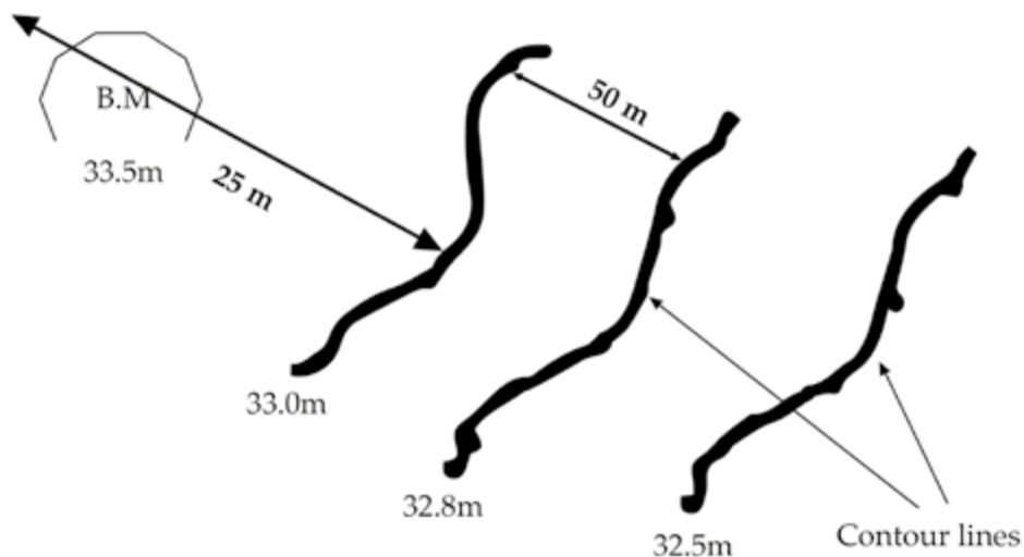
Figure 11.5: Using A-frame to map out contour lines
