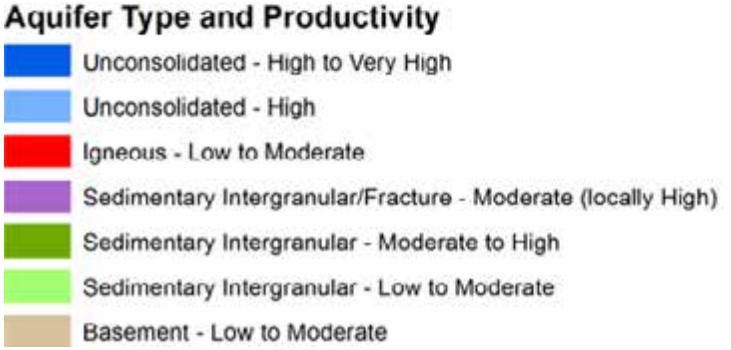
Figure 3.4: Example of a hydrogeological map showing aquifer productivity in Nigeria (Source: http://earthwise.bgs.ac.uk/index.php/Hydrogeology_of_Nigeria )
