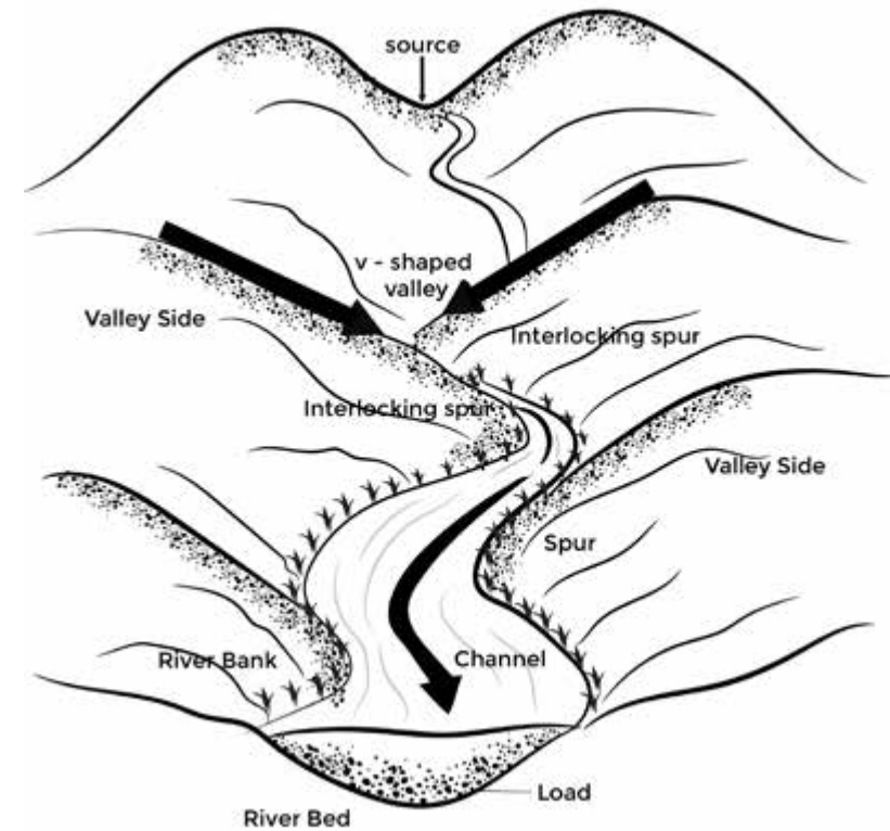
Figure 4.6: Sketch of stream course and landforms (Source: http://www.geography.learnontheinternet.co.uk/topics/river_upper_course.html )
