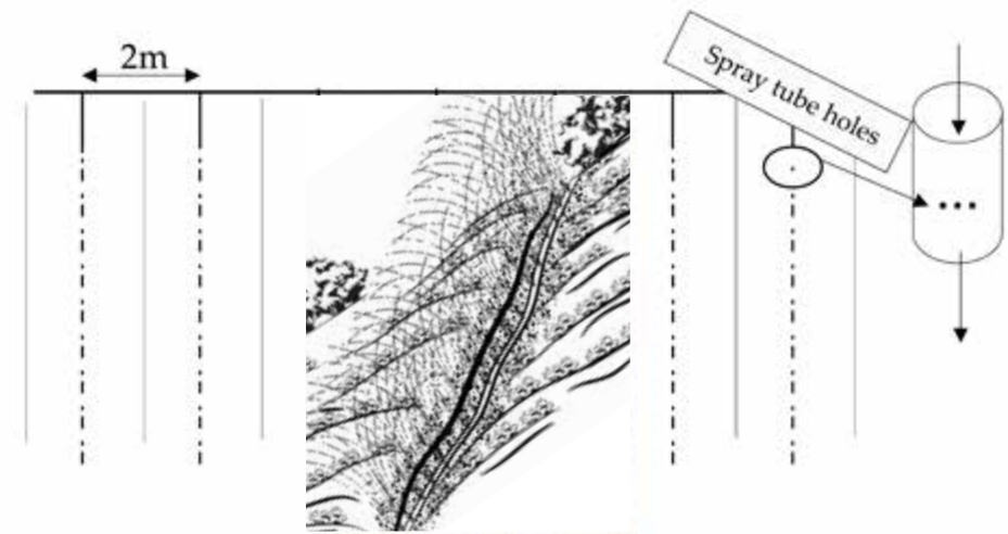
Figure 6.4: Rain tube installation
