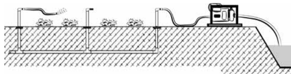
Figure 5.1: Buried Pipe Network system (Source: FAO, 2014)
