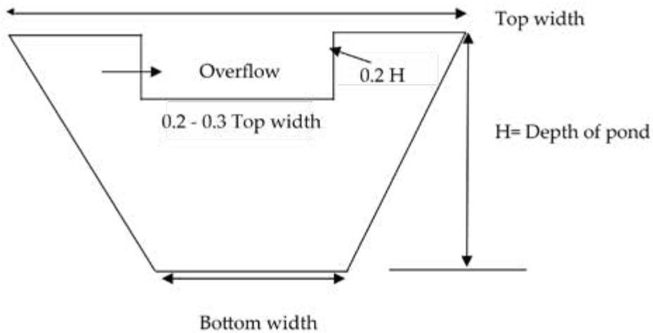
Figure 4.5: Side view of a typical farm pond with an overflow spillway
