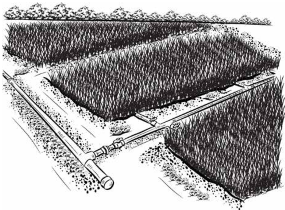
Figure 6.3: Rice production in check basin with piped water conveyance network
