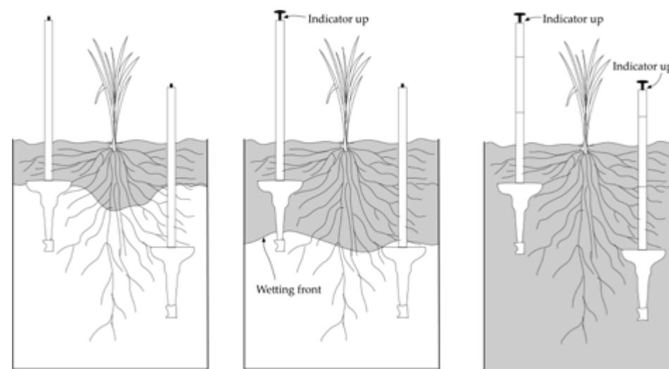
Figure 9.1: Typical use of wetting front detectors
