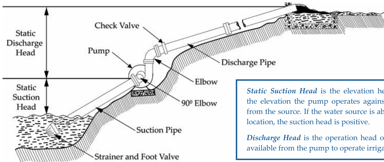
Figure 2.3: Basic layout of a typical surface water pumping (FAO, 1986)
