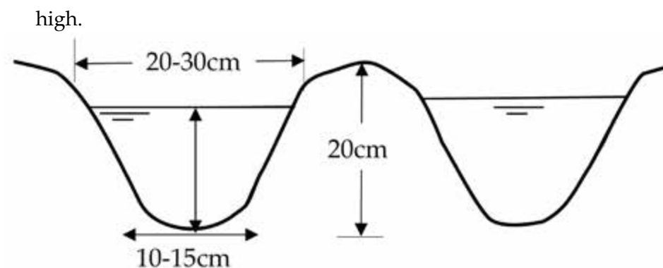
a. Deep narrow furrow on sandy soil
