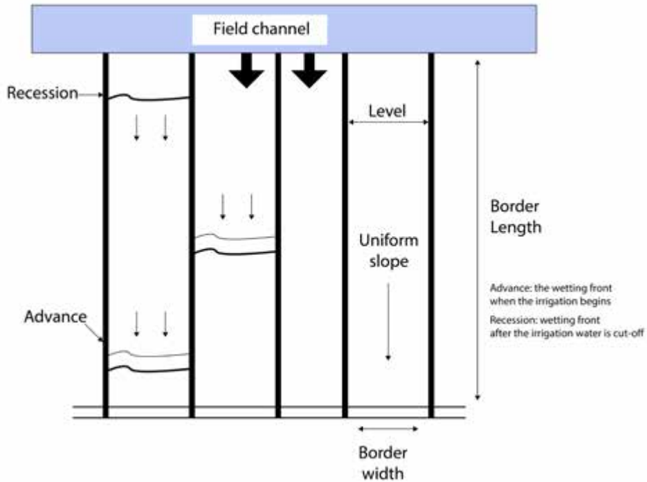
Figure 6.4: Border strips layout (Source: FAO, 2002)
