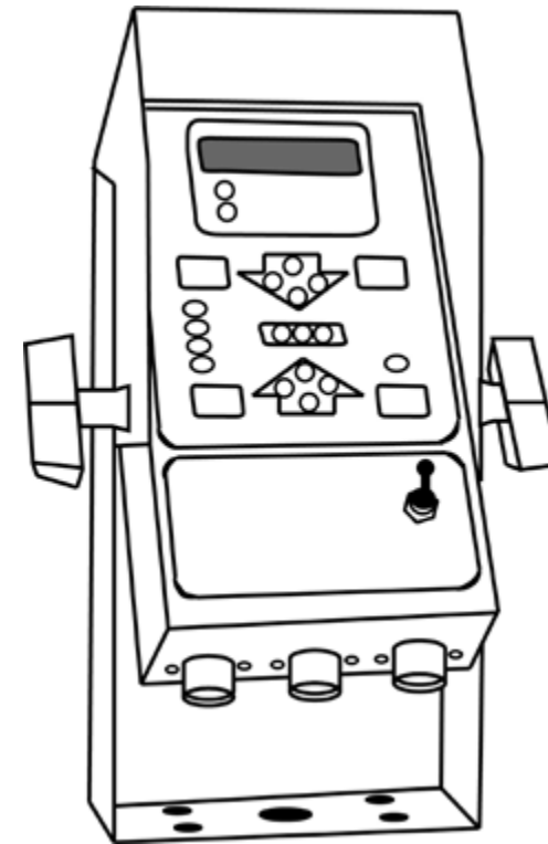
A view of the control panel (Source: https://www.meilaser.com/Laser-Machine-Control-Products )
