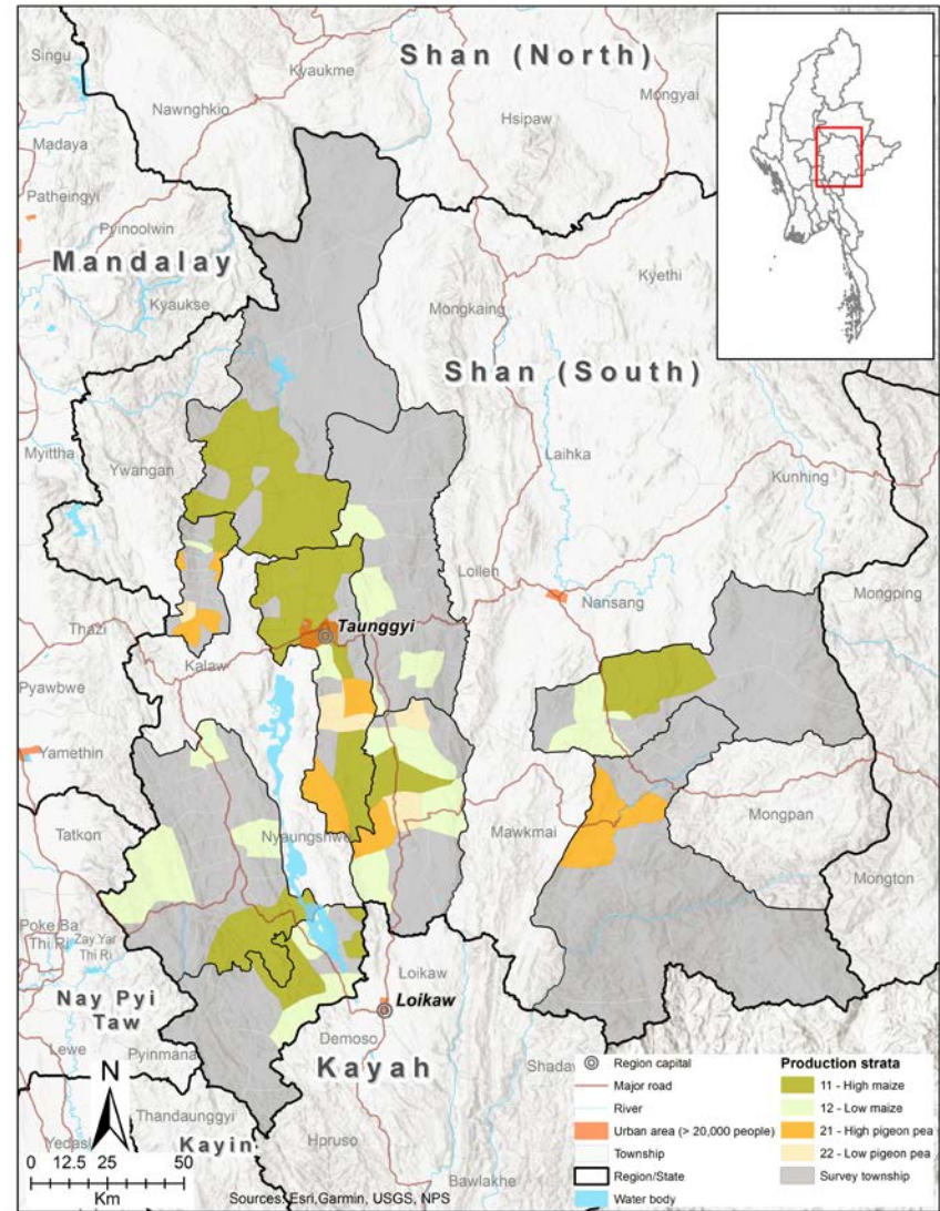
Figure 2 Sample strata
