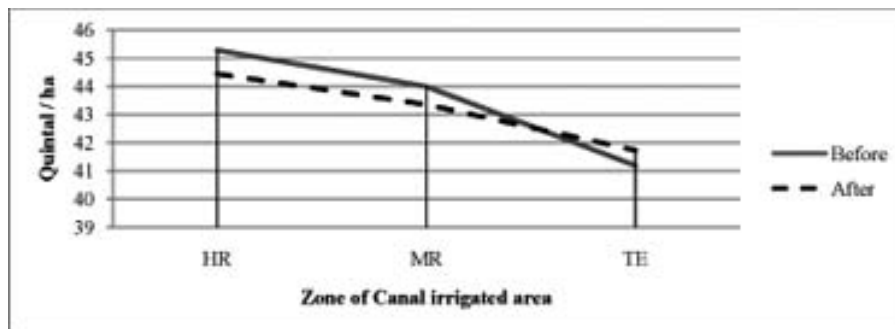
Figure 2. Average Monsoon Paddy Productivity Variation at Before and After Lock-Gate Regions.
