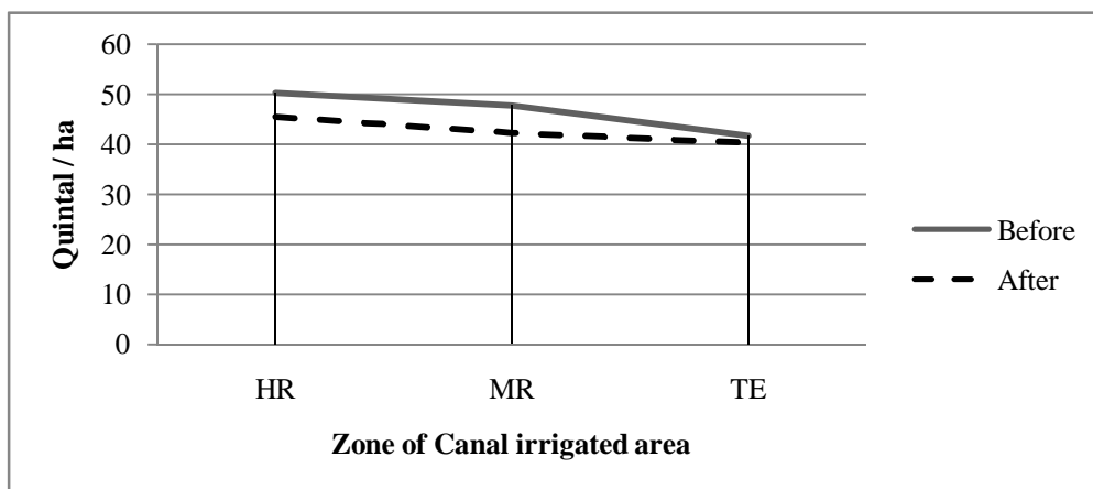
Figure 3. Average Boro Paddy Productivity Variation at Before and After Lock-Gate Regions.
