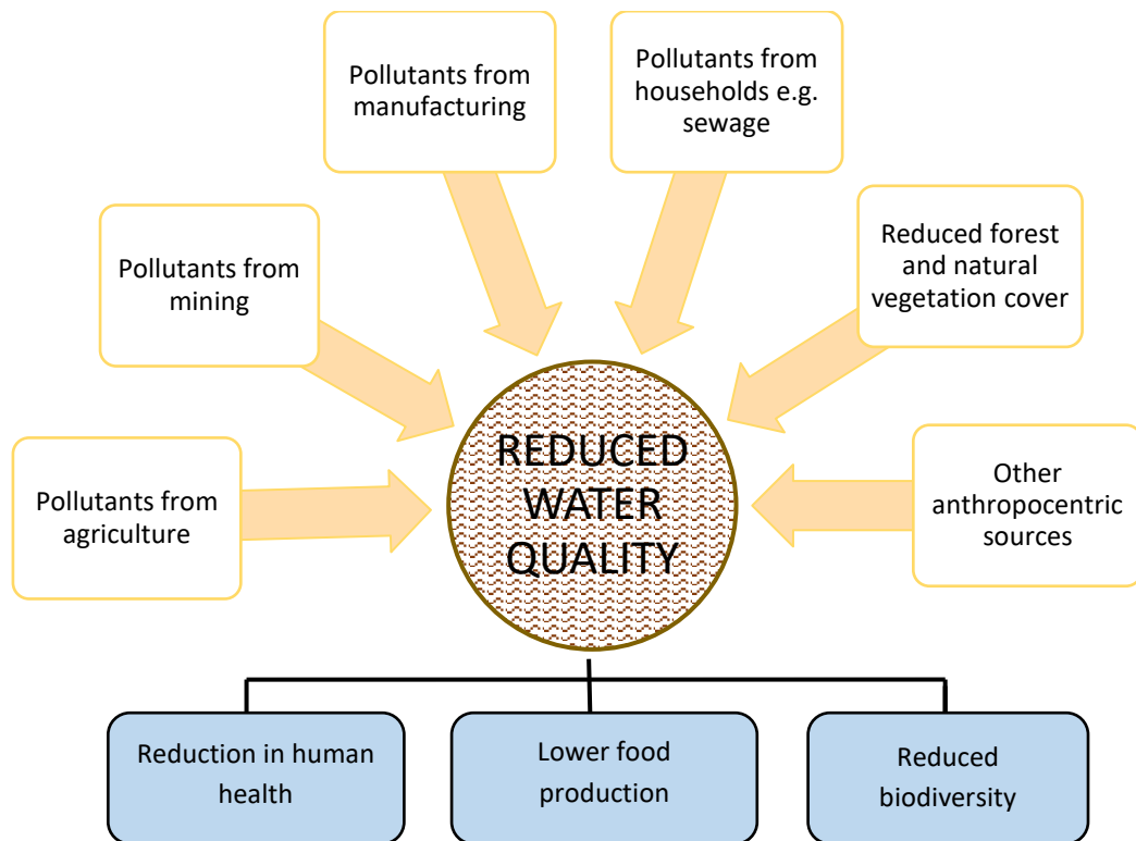
Fig 1: Multiple contributions to reduced water quality and consequences of water pollution. Note also that a reduction of water flows can add to the degree to which water is polluted.
