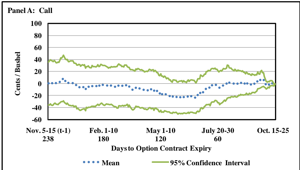
Figure 4. Gross Trading Return (Cents/Bushel), Long November Soybean Options, 1986-2009
