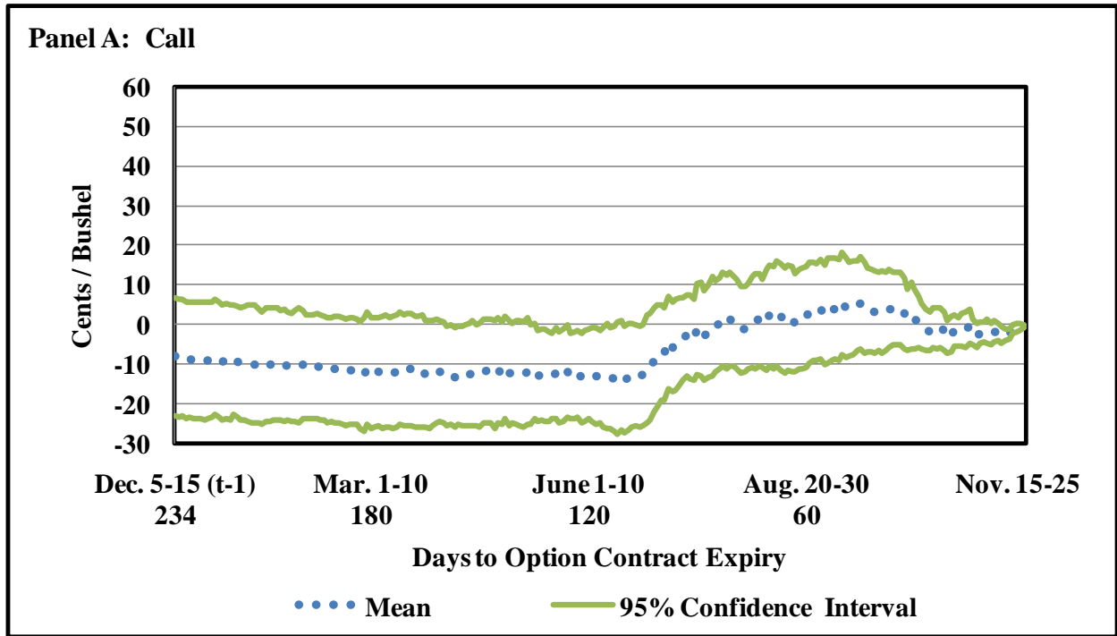
Figure 3. Gross Trading Return (Cents/Bushel), Long December Corn Options, 1986-2009
