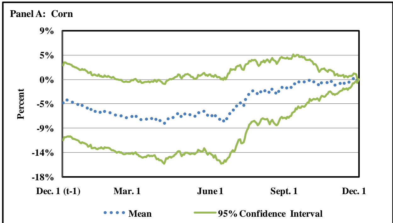
Figure 1. Gross Trading Return (Percent), Long December Corn Futures and Long November Soybean Futures, 1974-2009
