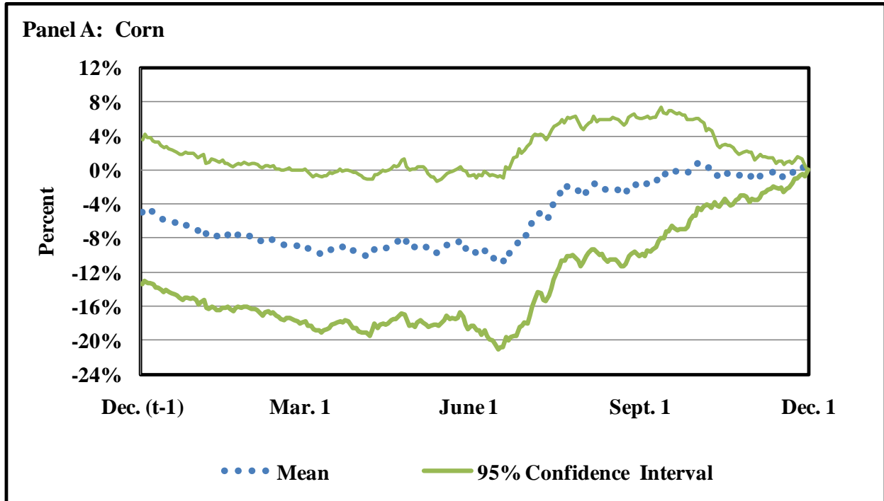
Figure 2. Gross Trading Return (Percent), Long December Corn Futures and Long November Soybean Futures, 1986-2009
