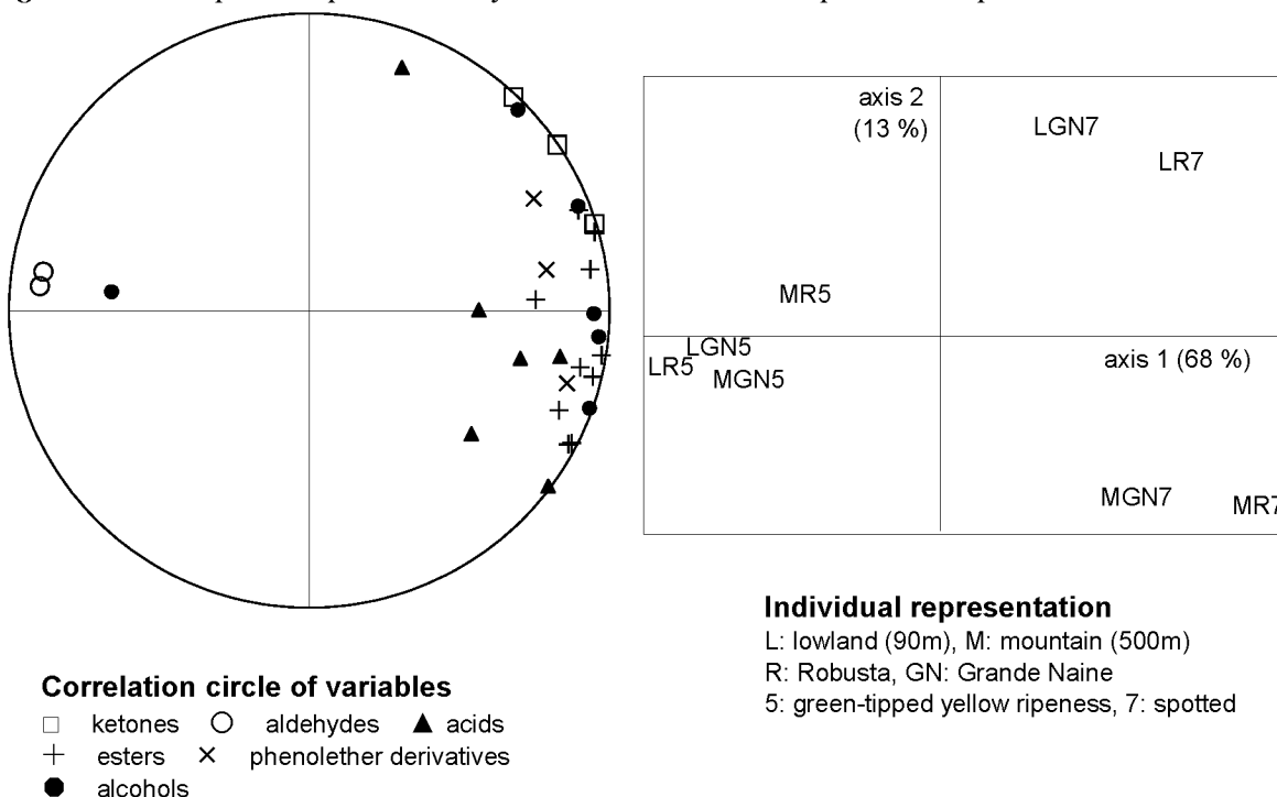
Figure 4: Principal component analysis of the volatile compound composition in bananas
