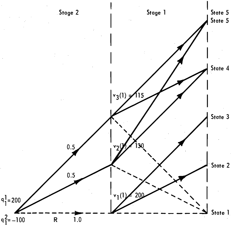
Fig. 1. Possible steps in two stages from state 1. The broken lines indicate replacement ( k = 2 ).
