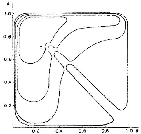
Fig. 11. Likelihood contours found by Model 2 for grain sorghum in the San Joaquin Valley
