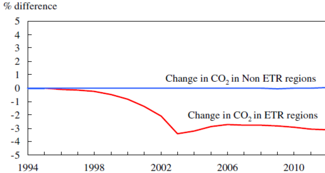
Figure 2 Changes in CO 2 emissions in the ETR and non-ETR countries (% difference between the base case and the counterfactual reference case) Source: Speck (2007).
