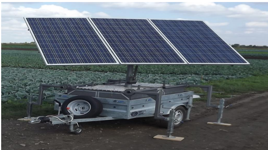
Picture 1. Mobile robotized solar electro-generator
