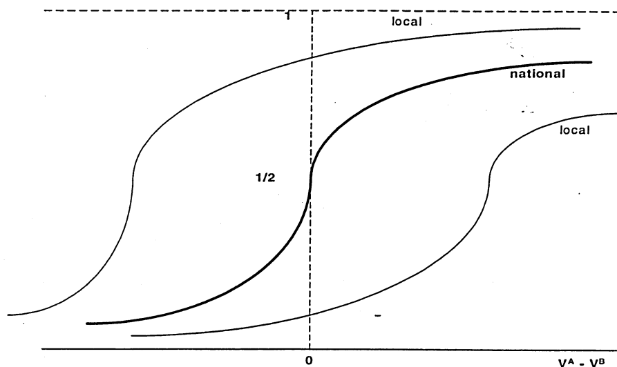
Figure 2: WIN PROBABILITIES AT LOCAL AND NATIONAL LEVELS WITH HETEROGENOUS PARTY PREFERENCES
