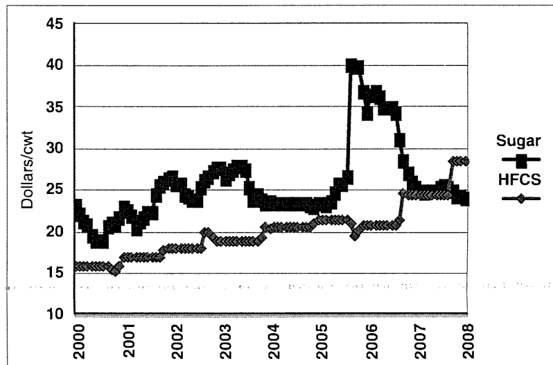
Figure 2. U.S. Wholesale Sugar and HFCS Price
