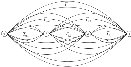
Figure 1. Dynamic programming network for the MSPATH
