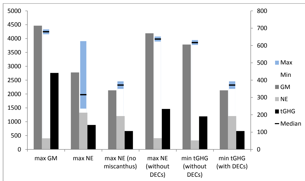
Figure 2: Outputs from the MEETA model in relation to the six scenarios. The black, dark grey and light grey columns (associated with the right hand axis) represent the total greenhouse gas emissions (tGHG, in 10s kg CO 2 eq ha -1 ), the gross margin (GM, £ ha -1 ) and the net farm energy (NE, GJ ha -1 ) for the farm for each of the scenarios. The blue box represents the max-min range of the water result for the scenario (associated with the left hand axis, m 3 ha -1 ) with the black line representing the median water use value for the scenario.
