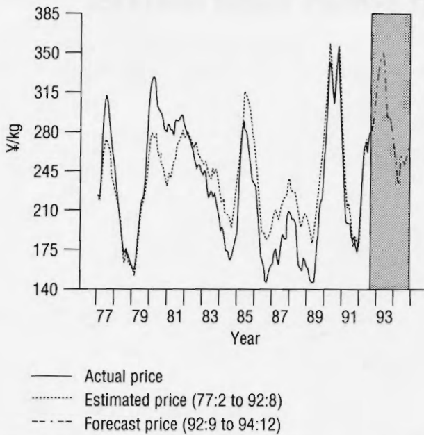
Figure 20.3 Skipjack price series and forecast: Yaizu fish market.
