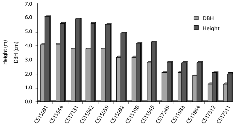
Figure 10. Growth performance, in terms of diameter at breast height over bark (DBH) and height, of species–provenances to age 3.5 years in the 1988 Chuxiong species–provenance trial II in Yunnan (Trial ID—Y8).
