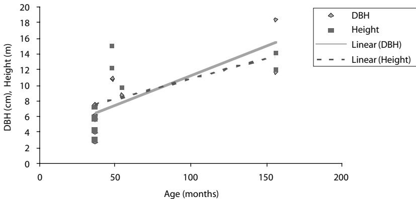
Figure 45. Growth of E. nitens across 10 sites on the Yunnan plateau.
