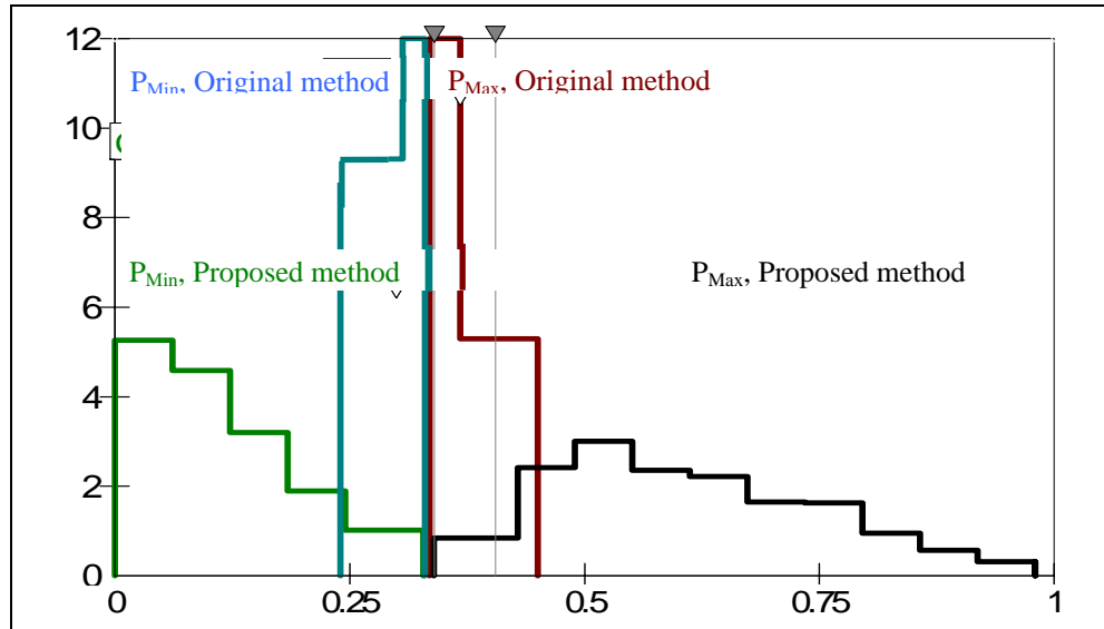
Figure 2: Distribution of initial probabilities: Original and proposed methods
